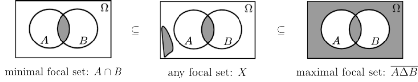
Fig. 1. Example of focal sets of mass function m_{A \cap B} .
